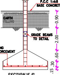
SECTION "E-E"
