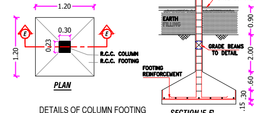
DETAILS OF COLUMN FOOTING
