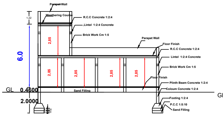
Section
