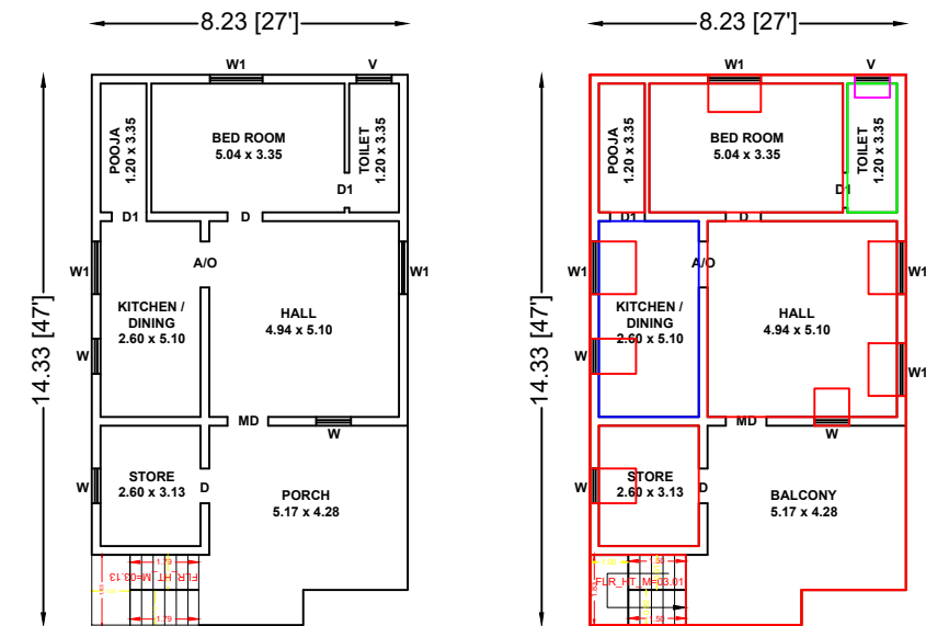
EXISTING GROUND FLOOR PLAN (EAST FACING)
