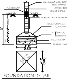
FOUNDATION DETAIL
