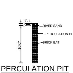
PERCOLATION PIT
