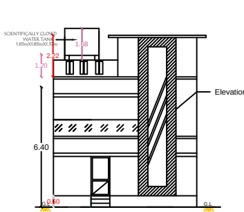
FRONT ELEVATION ( SOUTH FACING )
