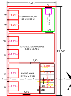
FLOOR PLAN ( NORTH FACING )
