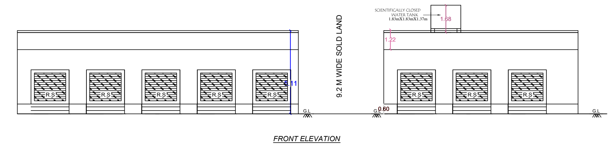
FRONT ELEVATION
