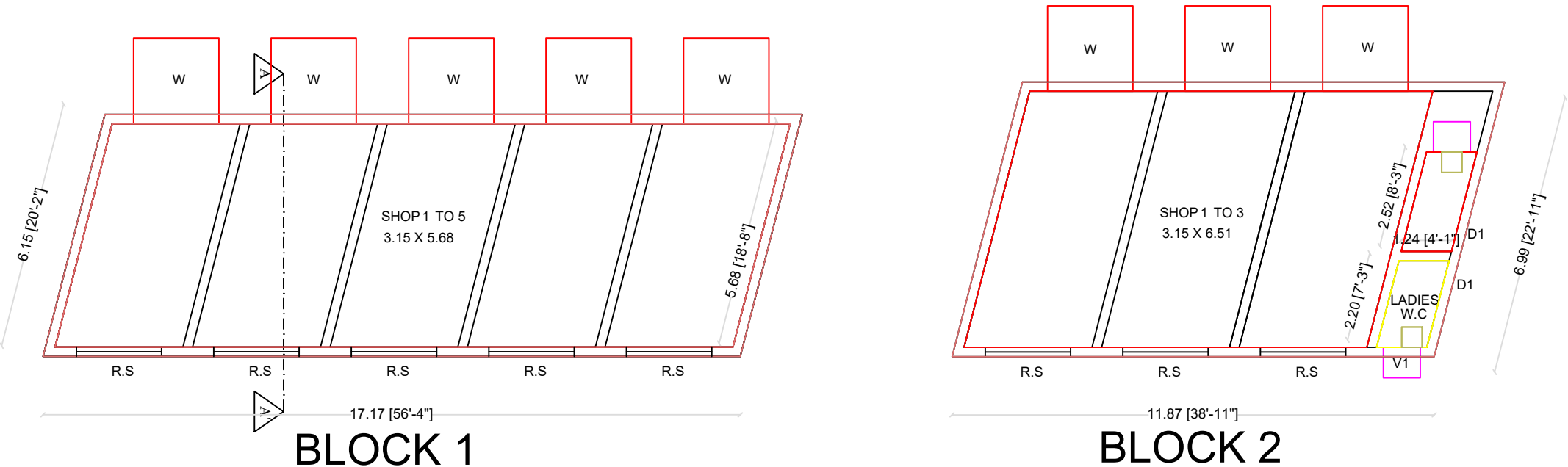
GROUND FLOOR PLAN -SOUTH FACING
