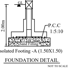
FOUNDATION DETAIL
