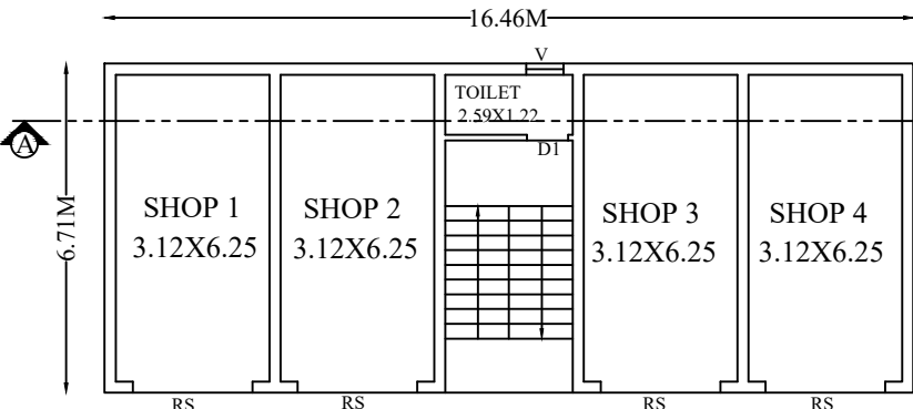
GROUND FLOOR PLAN (COMMERCIAL)
