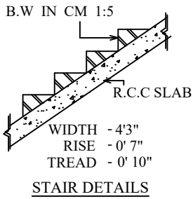
STAIR DETAILS
