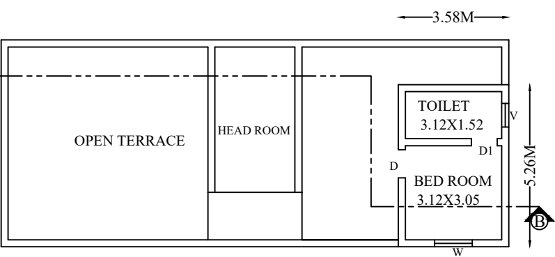
FIRST FLOOR PLAN (RESIDENTIAL)
