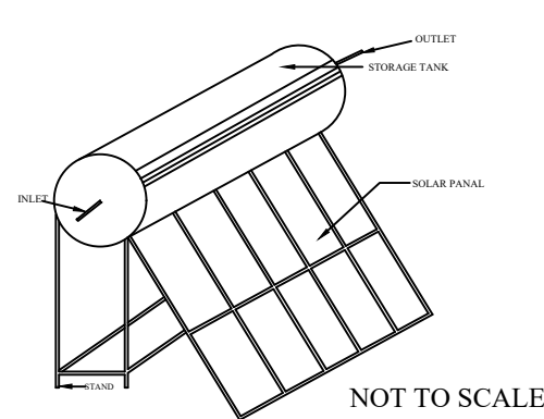
SOLAR WATER HEATER DETAILS
