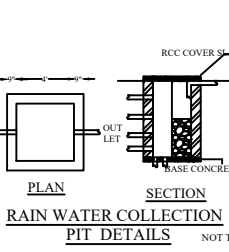
RAIN WATER COLLECTION PIT DETAILS
