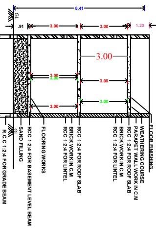
SECTION ON "B"
