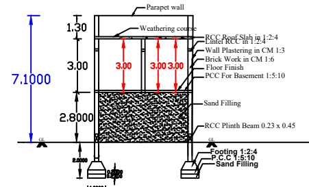
Section Section - AA
