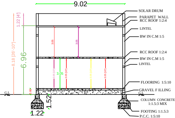
SECTION -RR
