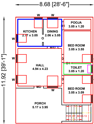
GROUND FLOOR PLAN (NORTH FACING)
