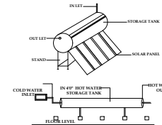
SOLAR HOT WATER SYSTEM DETAILS
