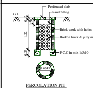
PERCOLATION PIT
