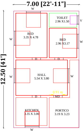
GROUND FLOOR PLAN EAST FACING
