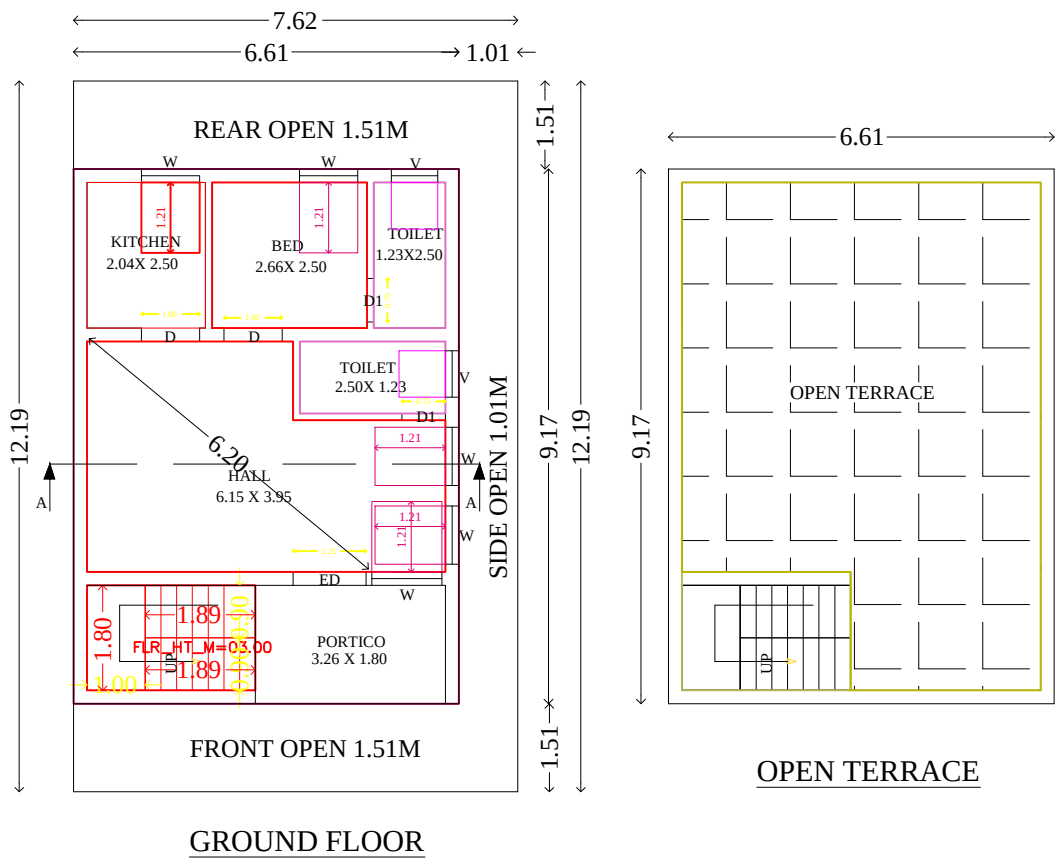
GROUND FLOOR
