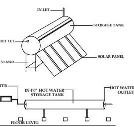
SOLAR HOT WATER SYSTEM DETAILS
