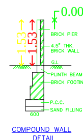
COMPOUND WALL DETAIL
