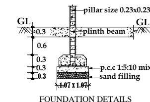
FOUNDATION DETAILS
