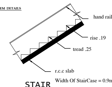
STAIR
