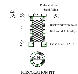
PERCOLATION PTT
