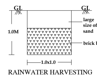
RAINWATER HARVESTING
