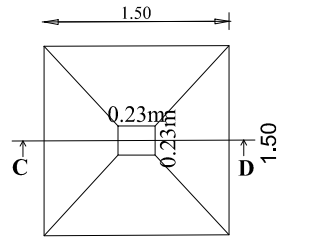
SECTION - 'CD' FOUNDATION DETAIL - A
