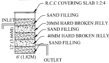
Waste Water Recycle Unit Not To Scale
