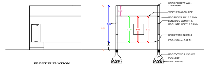
FRONT ELEVATION
