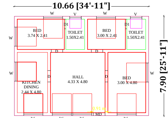
GROUND FLOOR PLAN EAST FACING
