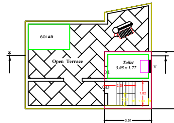
Proposed Terrace Floor Plan
