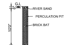
PERCOLATION PIT
