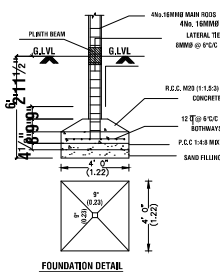
FOUNDATION DETAIL
