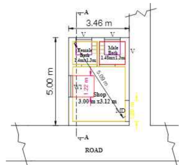
GROUND FLOOR PLAN [EAST FACING]
