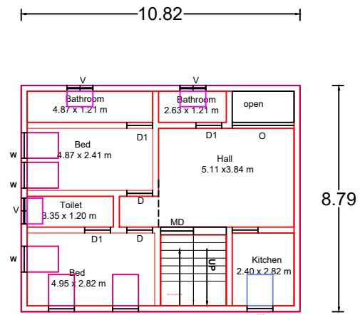
PROPOSED FIRST FLOOR PLAN ( SOUTH FACING )
