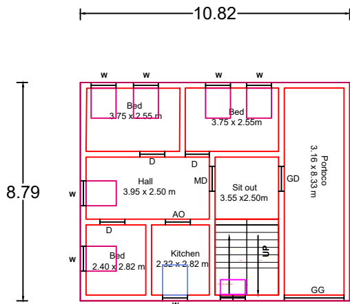
PROPOSED GROUND FLOOR PLAN ( SOUTH FACING )
