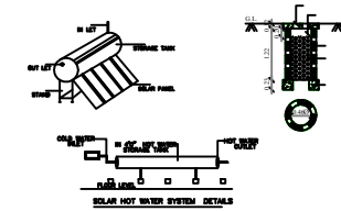
AREA DETAIL
