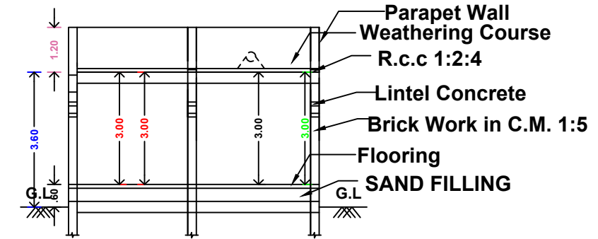
SECTION ON "BB"
