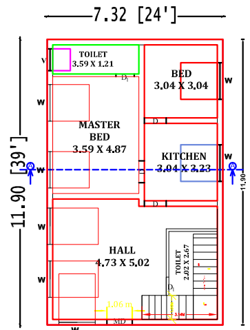
GROUND FLOOR PLAN (SOUTH FACING)
