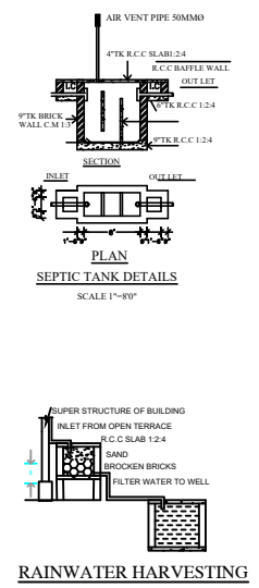
RAINWATER HARVESTING
