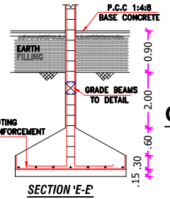
DETAILS OF COLUMN FOOTING
