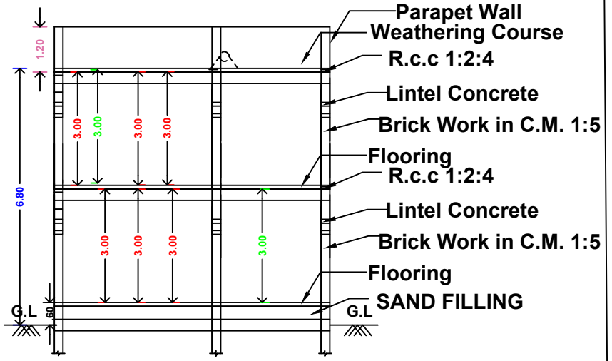
SECTION ON "BB"
