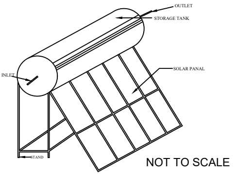
SOLAR WATER HEATER DETAILS
