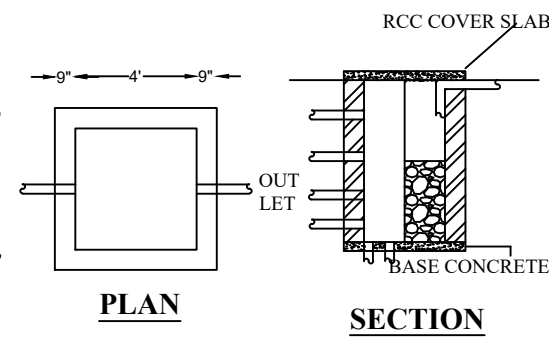
RAIN WATER COLLECTION PIT DETAILS
