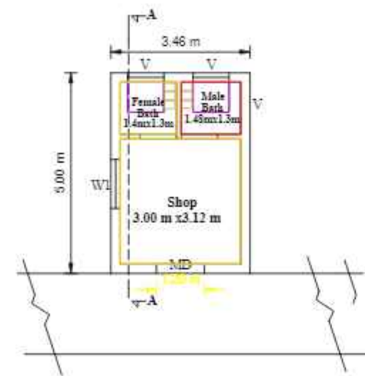
GROUND FLOOR PLAN [WEST FACING]
