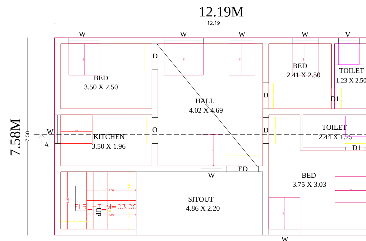
FIRST FLOOR (EAST FACHING)
