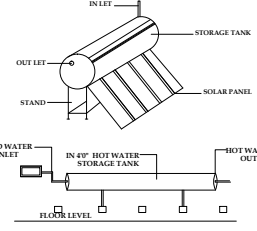
SOLAR HOT WATER SYSTEM DETAILS
