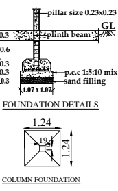
FOUNDATION DETAILS
