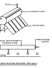
SOLAR HOT WATER SYSTEM DETAILS
