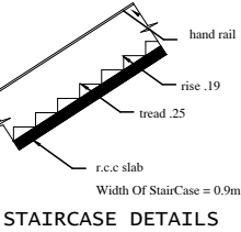
STAIRCASE DETAILS
