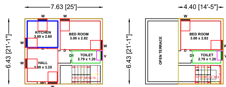
GROUND FLOOR PLAN (NORTH FACING)
