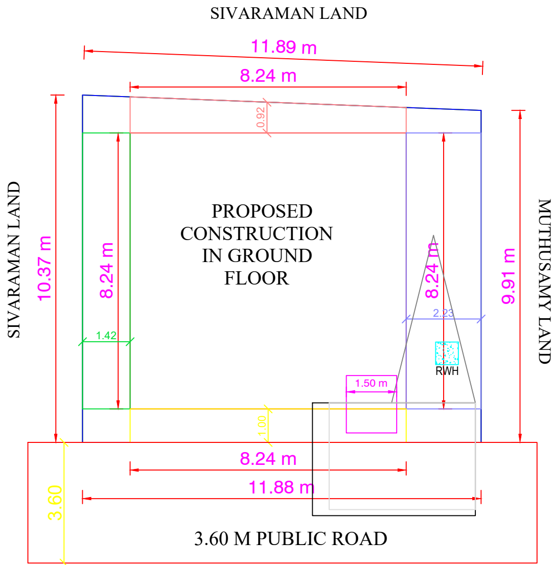
SITE PLAN
