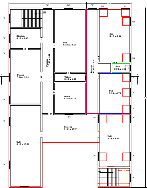
Existing & Proposed First Floor Plan
