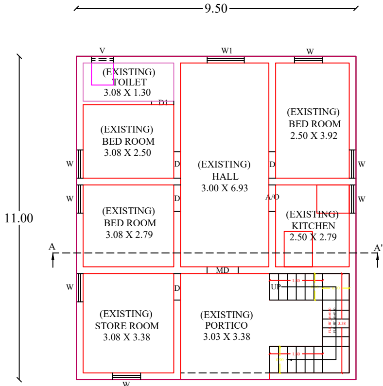
GROUND FLOOR PLAN (EXISTING BUILDING) (SOUTH FACING)
