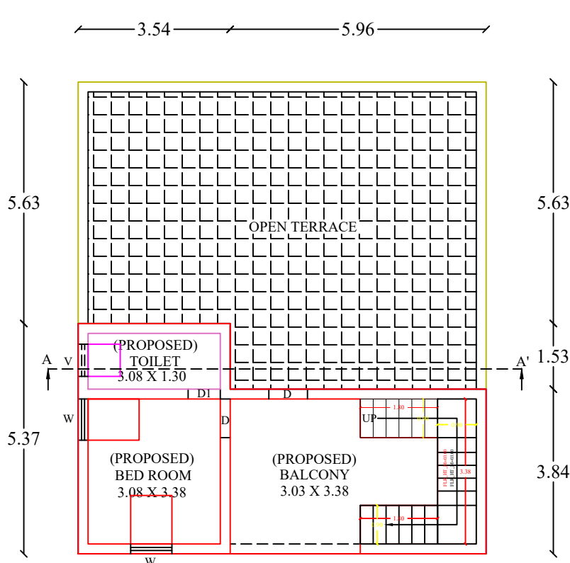
FIRST FLOOR PLAN (PROPOSED BUILDING)
