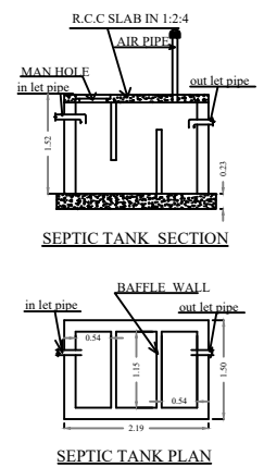
SEPTIC TANK DETAILS
