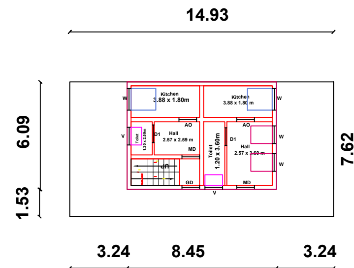
GROUND FLOOR PLAN EAST FACING
