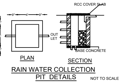
RAIN WATER COLLECTION PIT DETAILS
