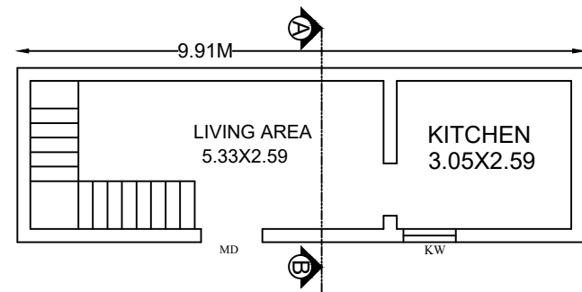
EXT.GROUND FLOOR PLAN
