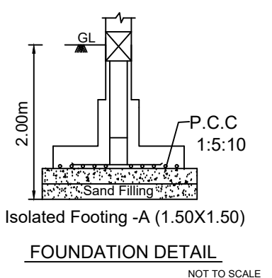
FOUNDATION DETAIL
