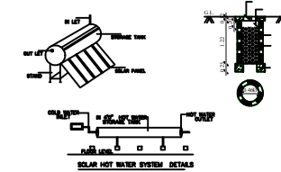
SOLAR HOT WATER SYSTEM DETAILS
