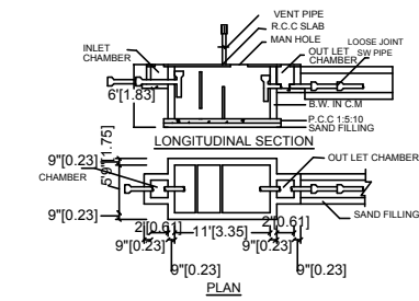
SEPTIC TANK DETAIL
