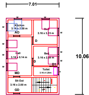
GROUND FLOOR PLAN (NORTH FACING)
