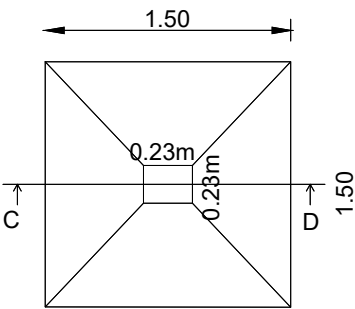
SECTION - 'CD'
