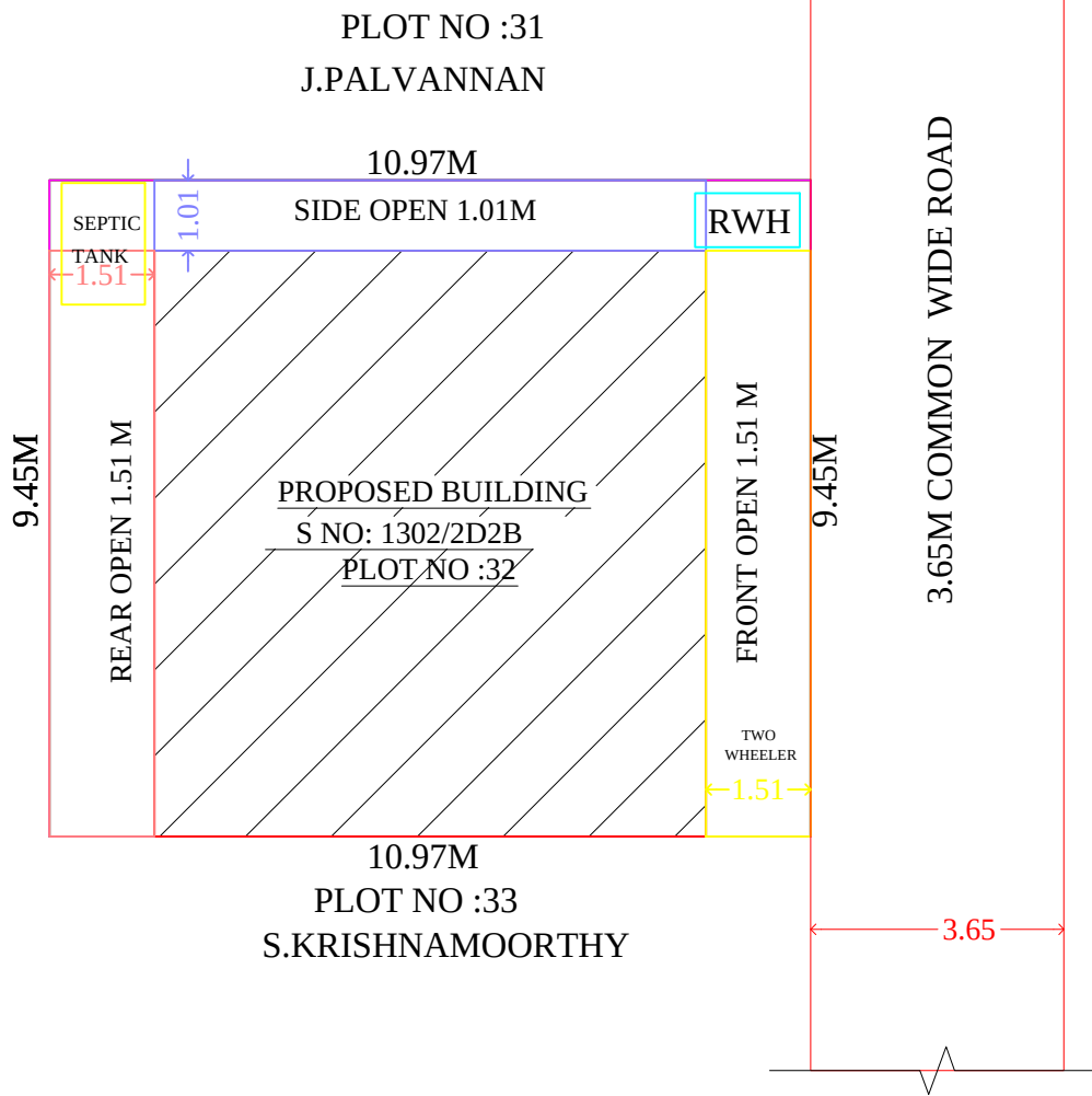
SITE PLAN
