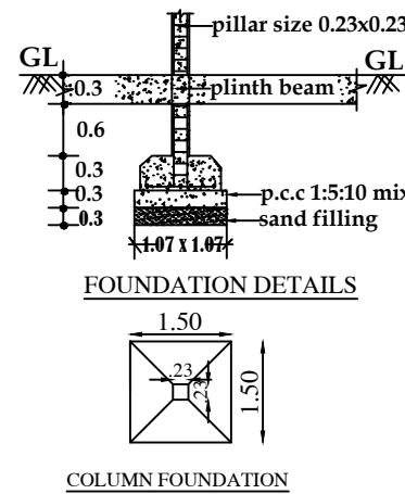
COLUMN FOUNDATION
