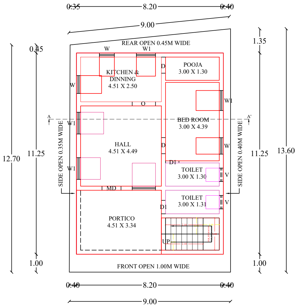
GROUND FLOOR PLAN (NORTH FACING)
