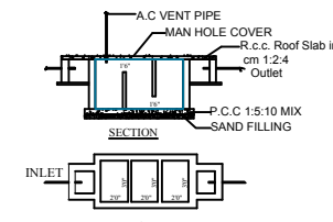
PLAN DETAILS OF SEPTIC TANK (Not to scale)
