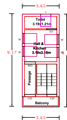
Pro.Second Floor Plan
