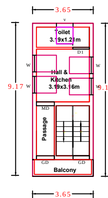
Pro.First Floor Plan
