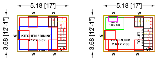
GROUND FLOOR PLAN (NORTH FACING)
