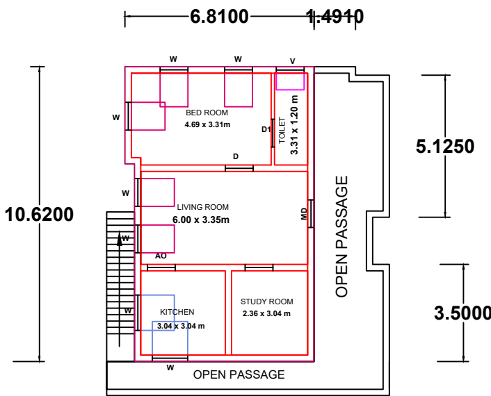
GROUND FLOOR PLAN ( EXISTING )
