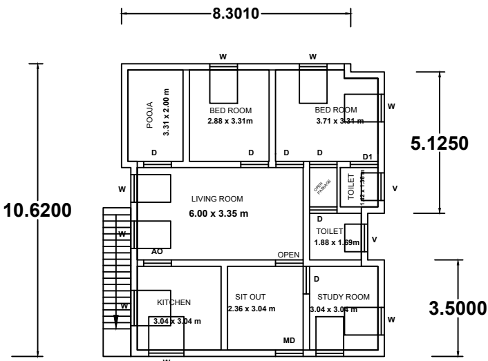
GROUND FLOOR PLAN ( EXISTING )
