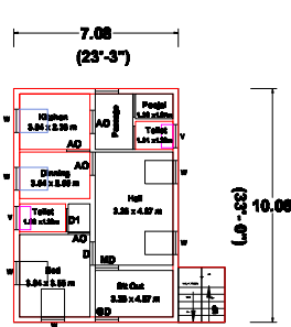
EXISTING GROUND FLOOR PLAN
