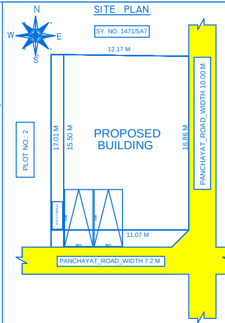
EAST - WEST STREET
