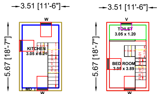
GROUND FLOOR PLAN (NORTH FACING)
