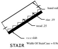
STAIR
