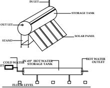
SOLAR HOT WATER SYSTEM DETAILS
